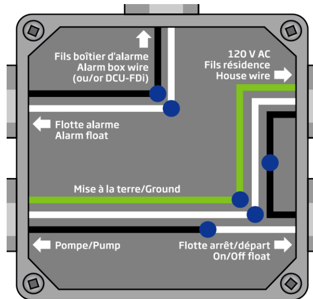
Electrical junction box
