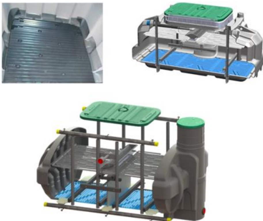
Figure 8. Planchers drainants
