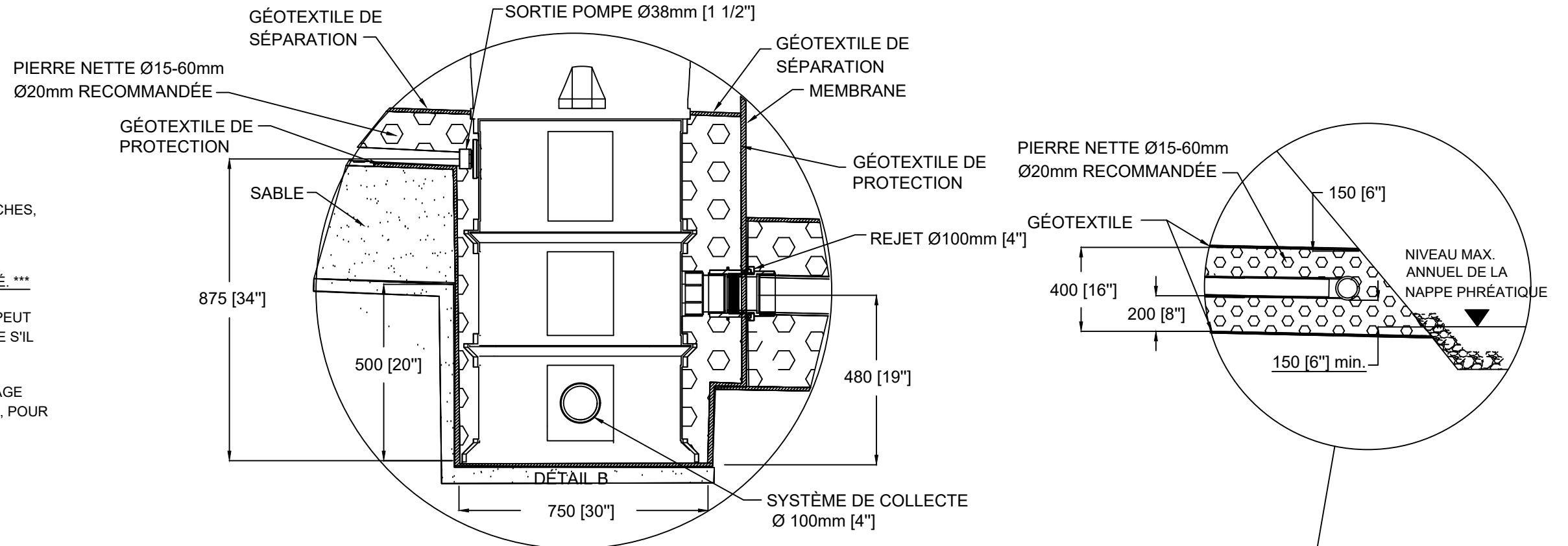
DETAIL B
