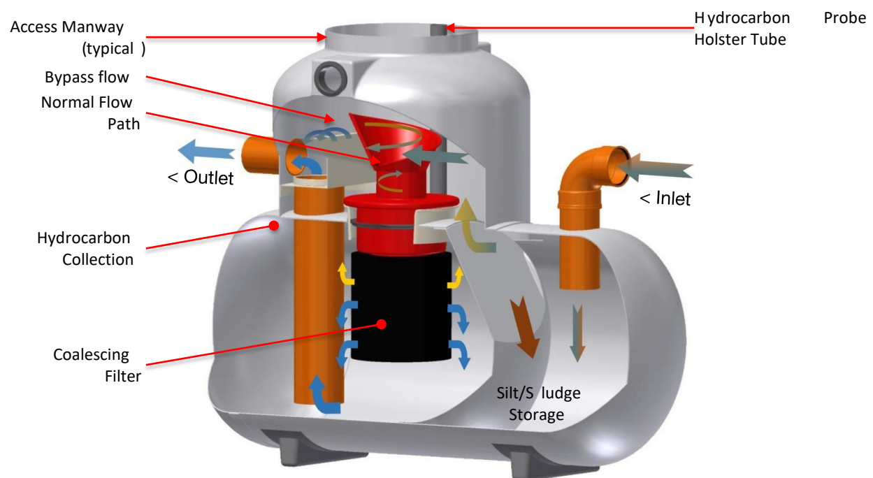
Figure 1: Bypass Separator
